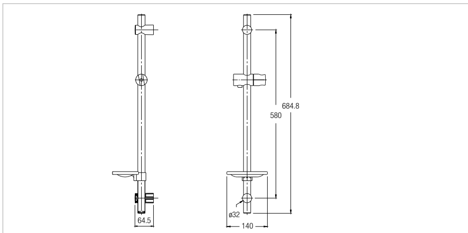
Technical drawings
