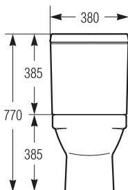
FRONT ELEVATION
